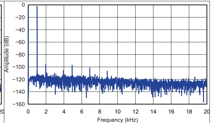
Figure 6. Line Input to ADC FFT Plot
