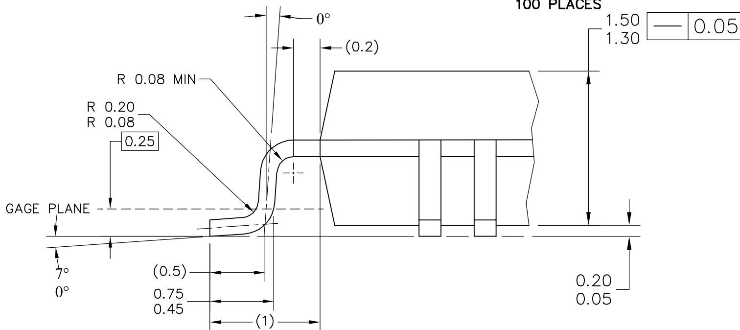
VIEW B
