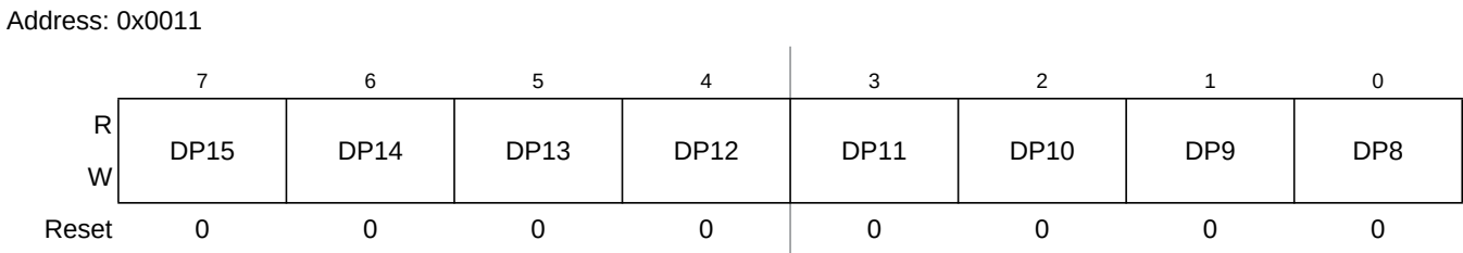
Figure 3-5. Direct Register (DIRECT)
