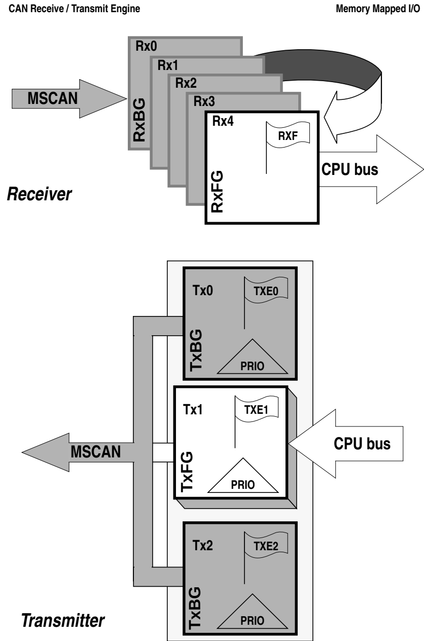
Figure 8-39. User Model for Message Buffer Organization
