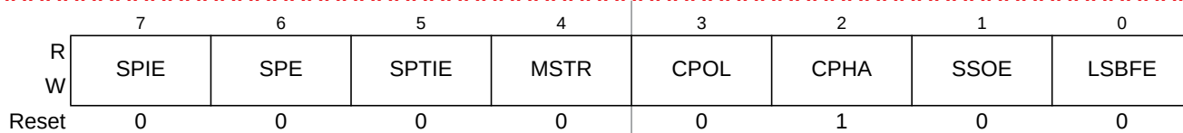
Figure 12-3. SPI Control Register 1 (SPICR1)
