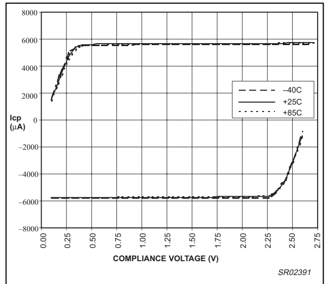
Figure 14. PHI_SU charge pump output vs. temperature (CP = 00_36x, V_{DD} = 3.0 V, Iset = 163 \mu A )
