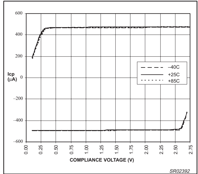
Figure 16. PHP charge pump output vs. temperature (CP = 10_3x, V_{DD} = 3.0 V, I_{set} = 163 \mu A )
