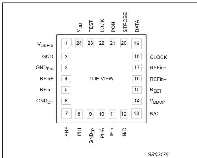
Figure 1. HBCC24 pin configuration.
