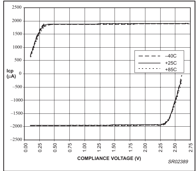
Figure 12. PHI_SU charge pump output vs. temperature (CP = 01_12x, V_{DD} = 3.0 V, Iset = 163 \mu A )
