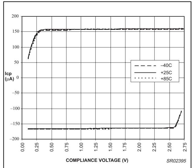
Figure 18. PHP charge pump output vs. temperature (CP = 11_1x, V_{DD} = 3.0 V, I_{set} = 163 \mu A )
