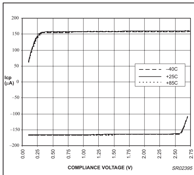
Figure 18. PHP charge pump output vs. temperature (CP = 11_1x, V DD = 3.0 V, Iset = 163 μA)
