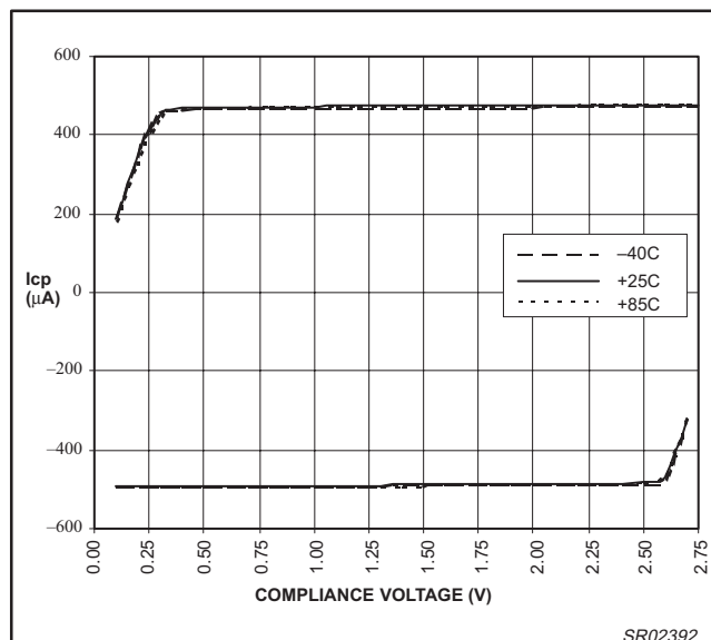
Figure 16. PHP charge pump output vs. temperature (CP = 10_3x, V DD = 3.0 V, Iset = 163 μA)
