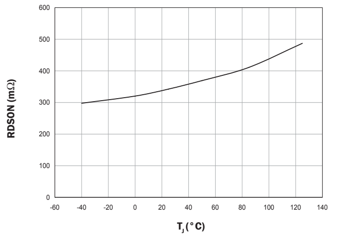
P-Channel R DSON vs. Temperature
