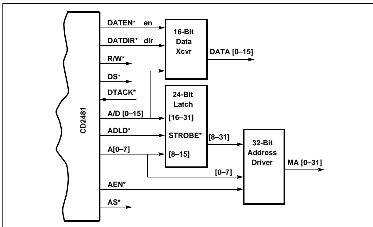
Figure 14. DMA Connections for the CD2481
