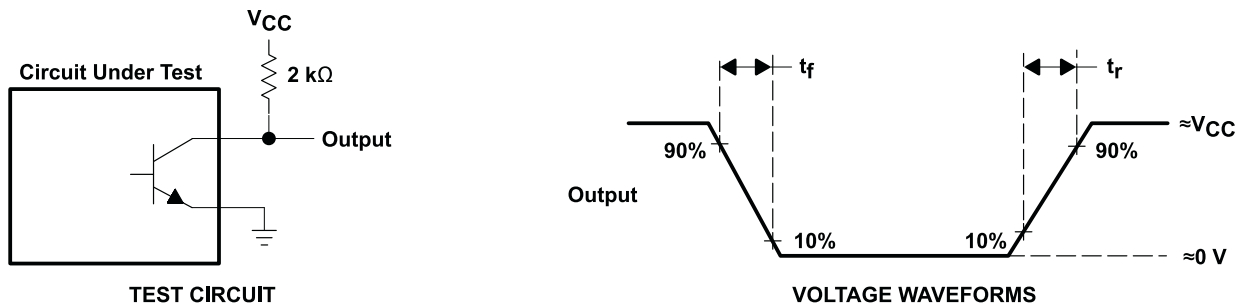
Figure 4. Switching Times
