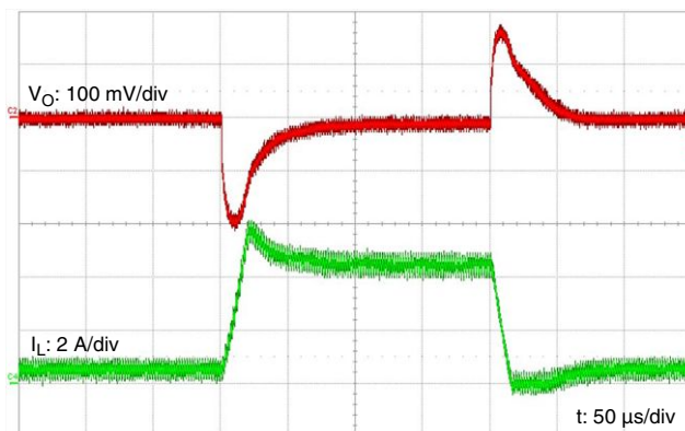
Transient response. V IN = 12 V, V O = 3.3 V and L = 10 μH (IHL P2525EZ type). C O consists of MLCC of 4.7 μF and tantalum of 100 μF/20 V x 2. Output current steps up and down between 0.4 A and 4 A with less than 1 μs rising and falling time.
