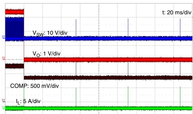
Overcurrent protection at I O = 8 ~ 10 A. V IN = 12 V, V O = 3.3 V and L = 10 μH (IHL P2525EZ type). C O consists of MLCC of 4.7 μF and tantalum of 100 μF/20 V x 2
