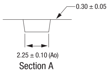
Figure 8. SC-88 Tape and Reel Dimensions
