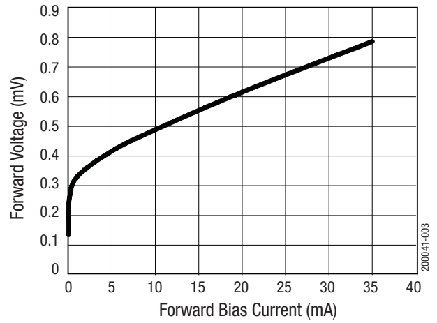
Figure 3. SMS7621 Forward Voltage vs Forward Bias Current
