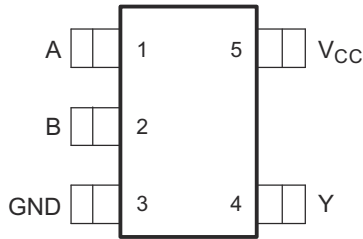
Figure 5-1. DBV Package SOT 5-pin (Top View)
