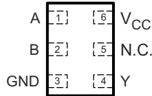
Figure 5-3. DSF Package SON 6-pin (Transparent Top View)
