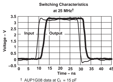
† AUP1G08 data at C_L = 15\text{ pF}
