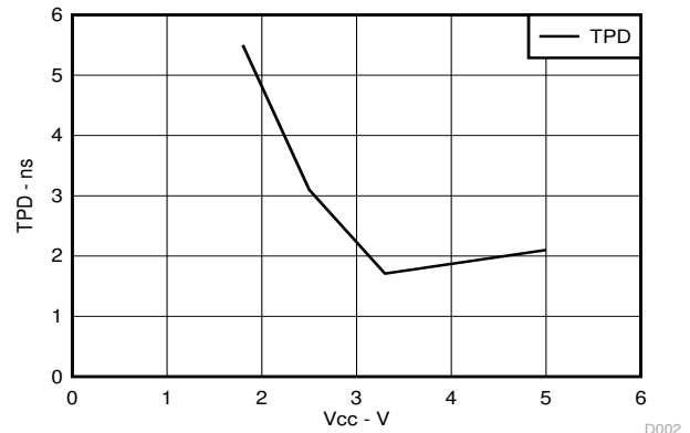
Figure 6-2. TPD Across Vcc at 25°C
