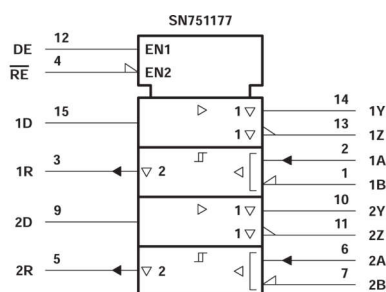
Logic Symbols †
