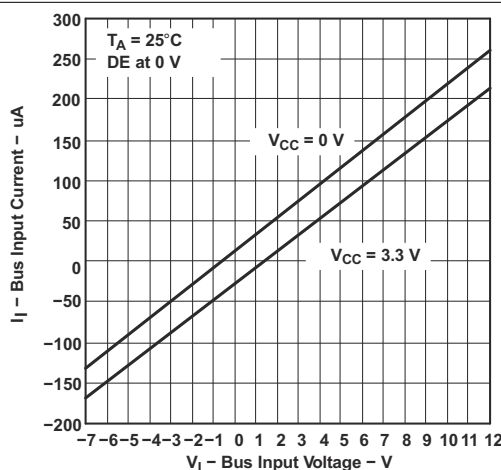
Figure 7-4. HVD10 Bus Input Current vs Bus Input Voltage
