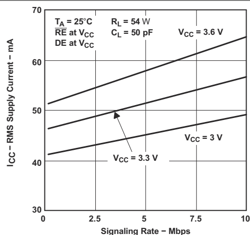
Figure 7-2. HVD11 RMS Supply Current vs Signaling Rate
