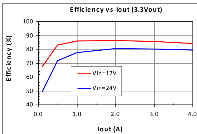
Figure 3- Efficiency, Natural convection at Vout=3.3V, Ta= 25°C
