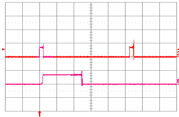
Fig. 6.0V.18: Load current (top trace, 20 A/div., 20 ms/div.) into a 10 \text{ m}\Omega short circuit during restart, at V_{in} = 24 \text{ V} . Bottom trace (20 A/div., 2 ms/div.) is an expansion of the on-time portion of the top trace.
