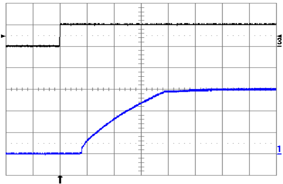
Fig. 6.0V.10: Turn-on transient at full rated load current (resistive) plus 10,000µF at V_{in} = 24\text{V} , triggered via ON/OFF pin. Top trace: ON/OFF signal (5 V/div.). Bottom trace: output voltage (2 V/div.). Time scale: 2 ms/div.
