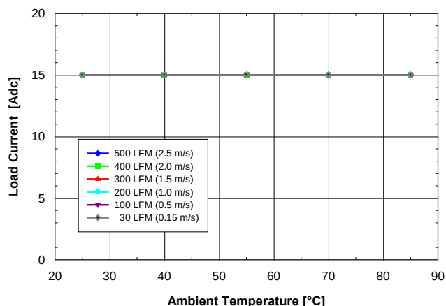
Fig. 1.2V.3: Available load current vs. ambient air temperature and airflow rates for SQ24S15012 converter mounted vertically with V_{in} = 24V , air flowing from pin 3 to pin 1 and maximum FET temperature \leq 120^{\circ}C .
