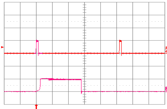
Fig. 3.3V.18: Load current (top trace, 20 A/div., 20 ms/div.) into a 10 \text{ m}\Omega short circuit during restart, at V_{in} = 24 \text{ V} . Bottom trace (20 A/div., 1 ms/div.) is an expansion of the on-time portion of the top trace.
