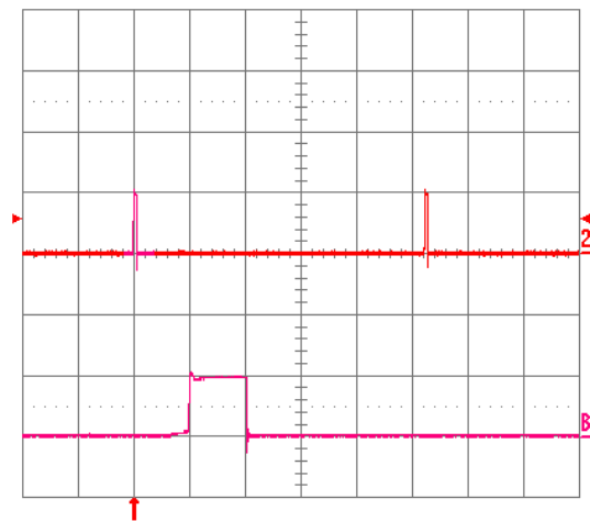
Fig. 1.5V.18: Load current (top trace, 20 A/div., 20 ms/div.) into a 10 m\Omega short circuit during restart, at V_{in} = 48 V. Bottom trace (20 A/div., 1 ms/div.) is an expansion of the on-time portion of the top trace.
