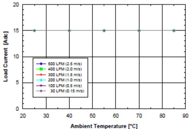
Fig. 1.0V.3: Available load current vs. ambient air temperature and airflow rates for SQ48S15010 converter mounted vertically with V_{in} = 48\text{ V} , air flowing from pin 3 to pin 1, and maximum FET temperature \leq 120\text{ }^{\circ}\text{C} .
