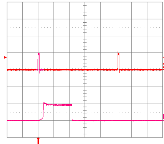
Fig. 3.3V.18: Load current (top trace, 20 A/div., 20 ms/div.) into a 10 mΩ short circuit during restart, at Vin = 48 V. Bottom trace (20 A/div., 1 ms/div.) is an expansion of the on-time portion of the top trace.
