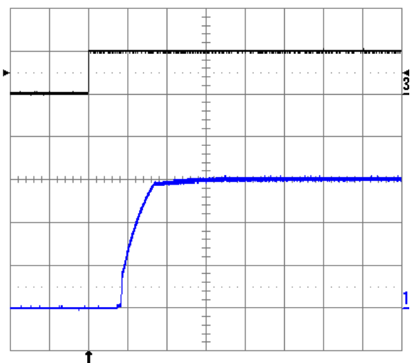
Fig. 1.5V.10: Turn-on transient at full rated load current (resistive) plus 10,000 \mu\text{F} at V_{in} = 48\text{ V} , triggered via ON/OFF pin. Top trace: ON/OFF signal (5 V/div.). Bottom trace: output voltage (0.5 V/div.). Time scale: 2 ms/div.
