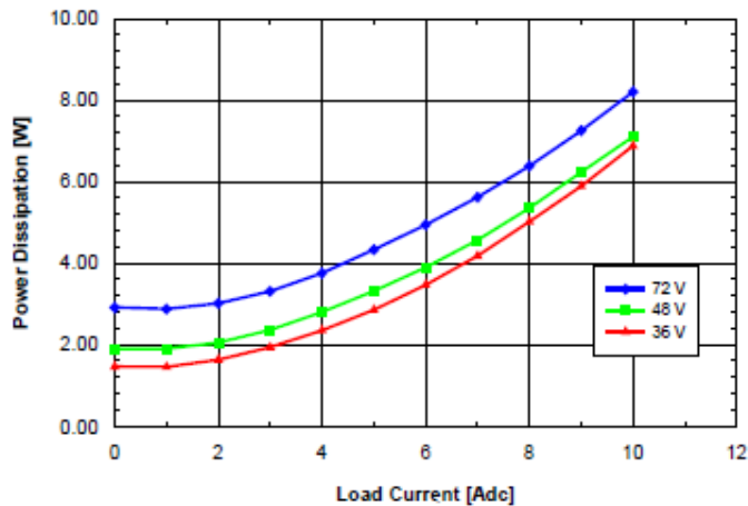
Fig. 5.0V.7: Power dissipation vs. load current and input voltage for SQ48T/S10050 converter mounted vertically with air flowing from pin 3 to pin 1 at a rate of 300 LFM (1.5 m/s) and T_a = 25^\circ\text{C} .
