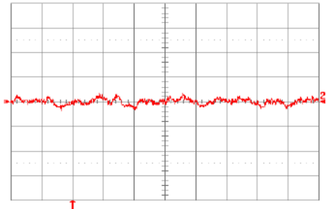
Fig. 6.0V.16: Input reflected ripple current, i_s (10 mA/div.), measured through 10\ \mu\text{H} at the source at full rated load current and V_{in} = 48\text{V} . Refer to Fig. 6.0V.14 for test setup. Time scale: 1 \mu\text{s} /div.
