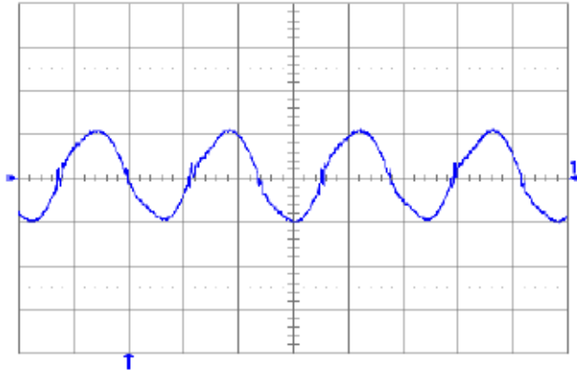
Fig. 5.0V.13: Output voltage ripple (20 mV/div.) at full rated load current into a resistive load with C_o = 10 \mu\text{F} tantalum + 1 \mu\text{F} ceramic and V_{in} = 48\text{V} . Time scale: 1 \mu\text{s}/\text{div} .
