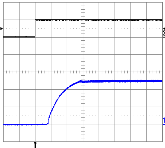
Fig. 2.5V.10: Turn-on transient at full rated load current (resistive) plus 10,000 \mu\text{F} at V_{in} = 48\text{ V} , triggered via ON/OFF pin. Top trace: ON/OFF signal (5 V/div.). Bottom trace: output voltage (1 V/div.). Time scale: 2 ms/div.
