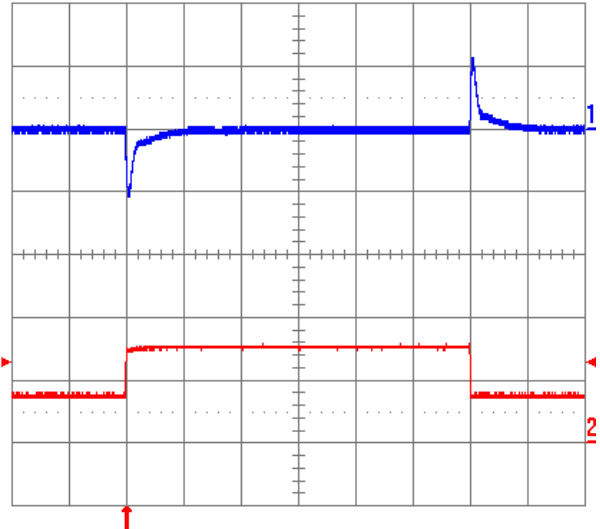
Fig. 1.5V.12: Output voltage response to load current step-change (3.75 A – 7.5 A – 3.75 A) at V_{in} = 48 V. Top trace: output voltage (100 mV/div.). Bottom trace: load current (5 A/div.). Current slew rate: 5 A/ \mu s. C_o = 450 \mu F tantalum + 1 \mu F ceramic. Time scale: 0.2 ms/div.
