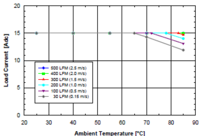
Fig. 1.8V.1: Available load current vs. ambient air temperature and airflow rates for SQ48T15018 converter with D height pins mounted vertically with V_{in} = 48\text{ V} , air flowing from pin 3 to pin 1, and maximum FET temperature \leq 120^\circ\text{C} .
