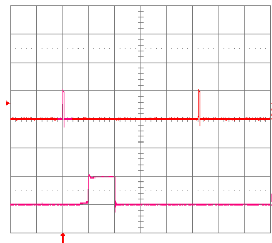
Fig. 1.5V.18: Load current (top trace, 20 A/div., 20 ms/div.) into a 10 m \Omega short circuit during restart, at V_{in} = 48 V. Bottom trace (20 A/div., 1 ms/div.) is an expansion of the on-time portion of the top trace.
