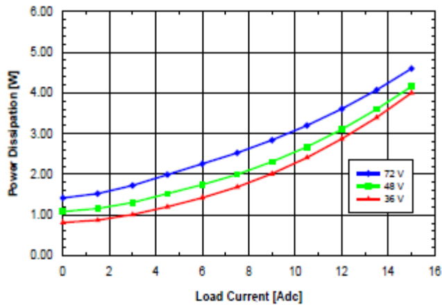
Fig. 1.5V.7: Power dissipation vs. load current and input voltage for SQ48T/S15015 converter mounted vertically with air flowing from pin 3 to pin 1 at a rate of 300 LFM (1.5 m/s) and T_a = 25^\circ\text{C} .
