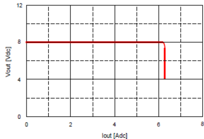
Fig. 8.0V.17: Output voltage vs. load current showing current limit point and converter shutdown point. Input voltage has almost no effect on current limit characteristic.
