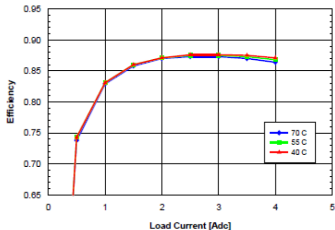
Fig. 12V.6: Efficiency vs. load current and ambient temperature for SQ48T/S04120 converter mounted vertically with V_{in} = 48V and air flowing from pin 3 to pin 1 at a rate of 200LFM (1.0 m/s).
