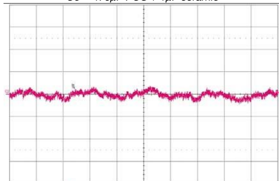
Figure 14. Input reflected-ripple current, i_s (10 mA/div.), measured through 10 \mu\text{H} at the source at full rated load current and V_{\text{in}} = 48\text{V} . Refer to Fig. J for test setup. Time scale: 1 \mu\text{s} /div.
