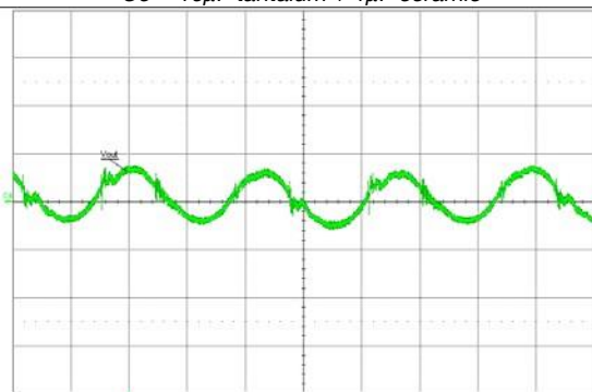
Figure 13. Output voltage ripple (20 mV/div.) at full rated load current into a resistive load with C_o = 10\mu\text{F} tantalum + 1 \mu\text{F} ceramic and V_{\text{in}} = 48\text{V} . Time scale: 1 \mu\text{s} /div.
