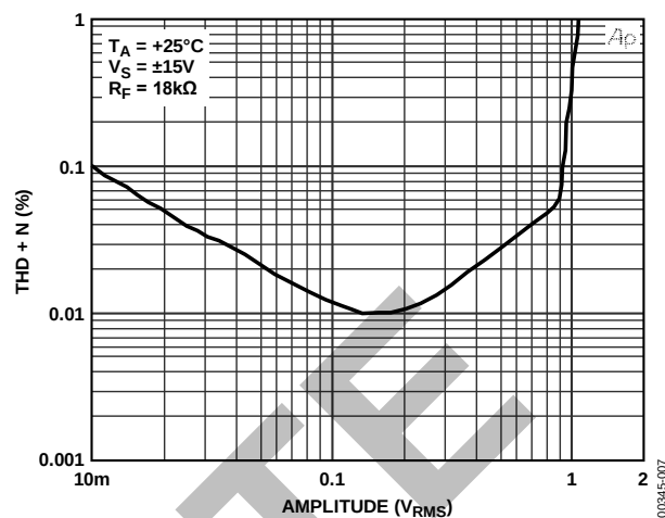
Figure 7. THD + N vs. Amplitude (Gain = +20\text{ dB} , f_{IN} = 1\text{ kHz} , 80 kHz Low-Pass Filter)
