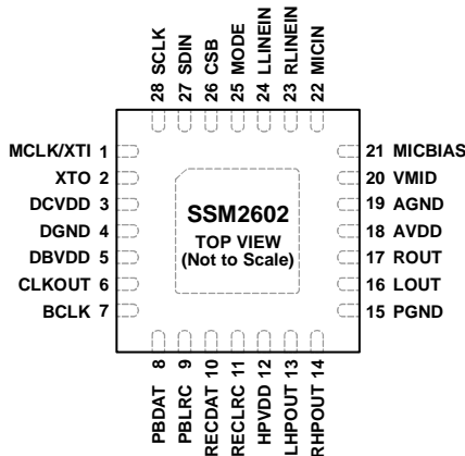
Figure 7. Pin Configuration
