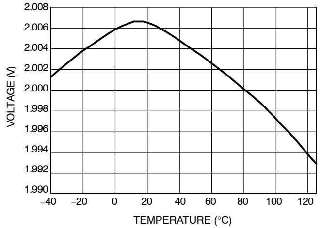
Figure 16. V LATCH
