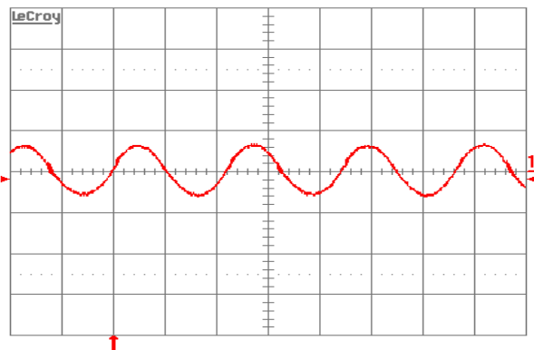
Figure 13: Input reflected-ripple-current, i_c (200 mA/div.), through 10 measured at input terminals at full rated load current and V_{in} = 48 \text{ V} . Refer to Figure 11 for test setup. Time scale: 1 \mu\text{s}/\text{div} .
