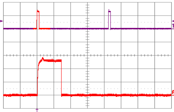
Figure 15: Load current (top trace, 20 A/div., 50 mS/div.) into a 10 mΩ short circuit during restart, at V_{in} = 48 \text{ V} . Bottom trace (10 A/div. 5 mS/div.) is an expansion of the on-time portion of the top trace.
