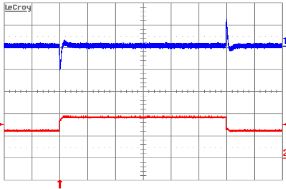
Figure 9. Output voltage response to load current step-change (12.5A–18.75A–12.5A) at V_{in} = 48\text{ V} . Top trace: output voltage (100 mV/div.). Bottom trace: load current (10A/div.). Current
