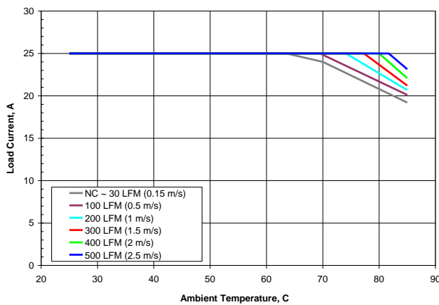
Figure 1. Available load current vs. ambient air temperature and airflow rates for SSQE48T25012 converter mounted vertically with air flowing from pin 1 to pin 3, V_{in} = 48\text{ V} . Note: NC - Natural convection
