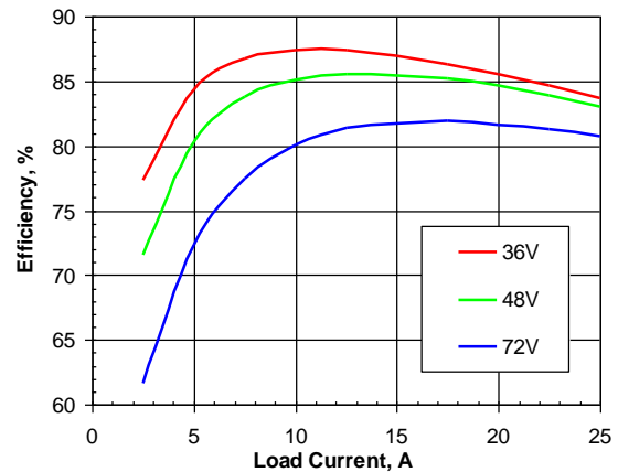
Figure 2. Efficiency vs. load current and input voltage for SSQE48T25012 converter mounted vertically with air flowing from pin 1 to pin 3 at a rate of 300 LFM (1.5 m/s) and T_a=25^\circ\text{C} .
