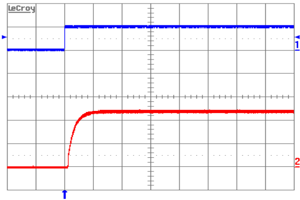
Figure 6. Turn-on transient at full rated load current (resistive) with C_o = 1\mu\text{F cer} + 10\mu\text{F tant} at V_{in} = 48\text{ V} , triggered via ON/OFF pin. Top trace: ON/OFF signal (5 V/div.). Bottom trace: Output voltage (0.5 V/div.). Time scale: 5 ms/div.
