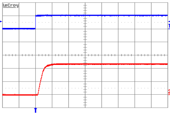
Figure 7. Turn-on transient at full rated load current (resistive) plus 30,000 \mu\text{F} at V_{in} = 48\text{ V} , triggered via ON/OFF pin. Top trace: ON/OFF signal (5 V/div.). Bottom trace: Output voltage (0.5 V/div.). Time scale: 5 ms/div.
