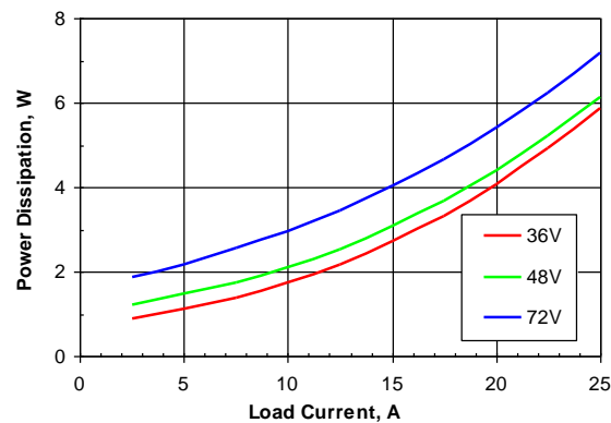
Figure 4. Power dissipation vs. load current and input voltage for SSQE48T25012 converter mounted vertically with air flowing from pin 1 to pin 3 at a rate of 300 LFM (1.5 m/s) and T_a = 25^\circ\text{C} .
