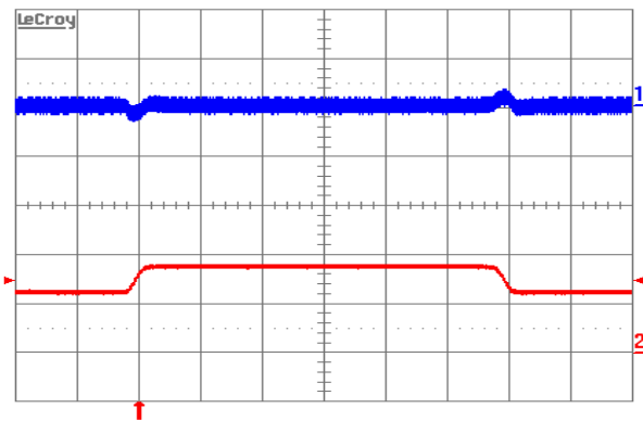
Figure 8. Output voltage response to load current step-change (12.5A–18.75A–12.5A) at V_{in} = 48\text{ V} . Top trace: output voltage (100mV/div.). Bottom trace: load current (10A/div.). Current slew rate: 0.1\text{ A}/\mu\text{s} . C_o = 1\mu\text{F cer} + 10\mu\text{F tant} . Time scale: 0.2ms/div.
