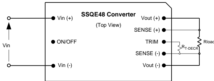
Figure D. Configuration for decreasing output voltage.
