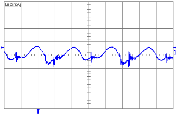
Figure 10. Output voltage ripple (20 mV/div.) at full rated load current into a resistive load with C_o = 10\mu\text{F tantalum} + 1\mu\text{F} slew rate: 5\text{ A}/\mu\text{s} . C_o = 470\mu\text{F POS} + 1\mu\text{F cer. ceramic} and V_{in} = 48\text{ V} . Time scale: 1\mu\text{s}/\text{div} . Time scale: 0.2ms/div.
