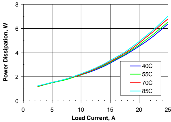
Figure 5. Power dissipation vs. load current and ambient temperature for SSQE48T25012 converter mounted vertically with V_{in} = 48\text{ V} and air flowing from pin 1 to pin 3 at a rate of 200 LFM (1.0 m/s).
