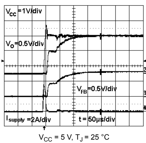
Figure 21. Startup transient
