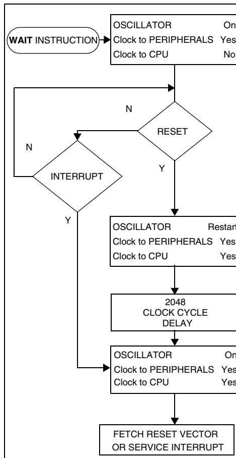
Figure 20. WAIT Mode Flowchart
