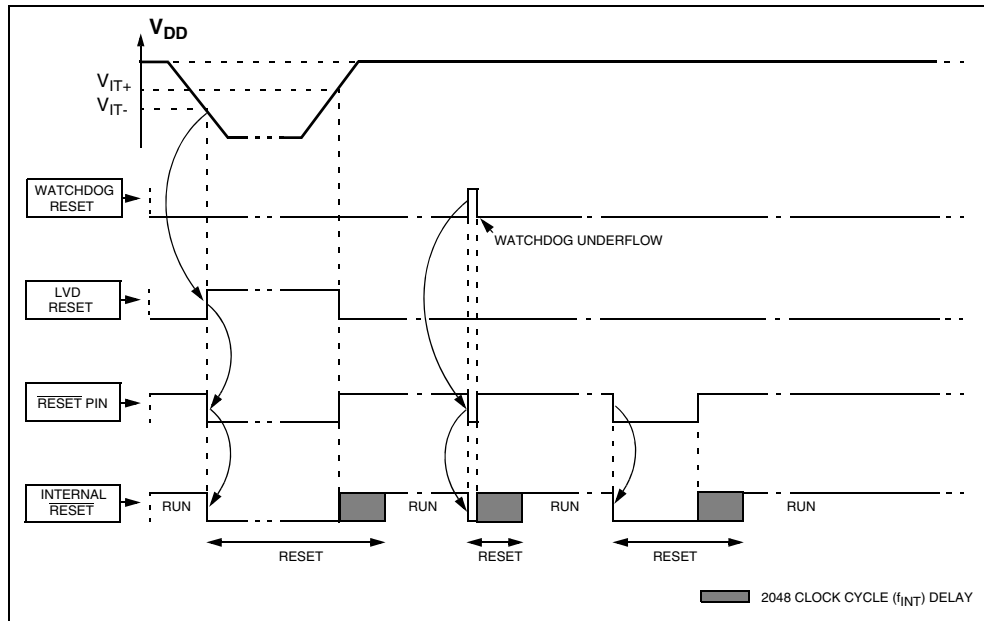
Figure 13. RESET Sequence
