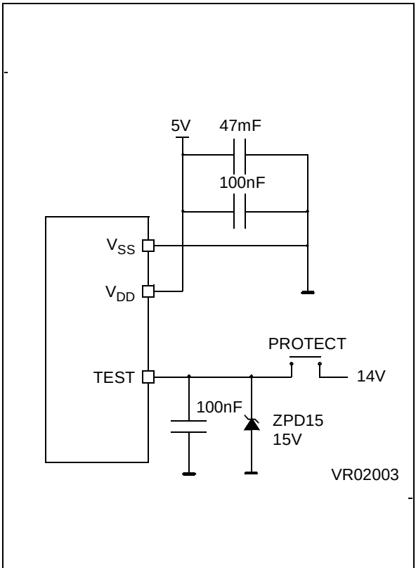
Figure 55. Programming Circuit
