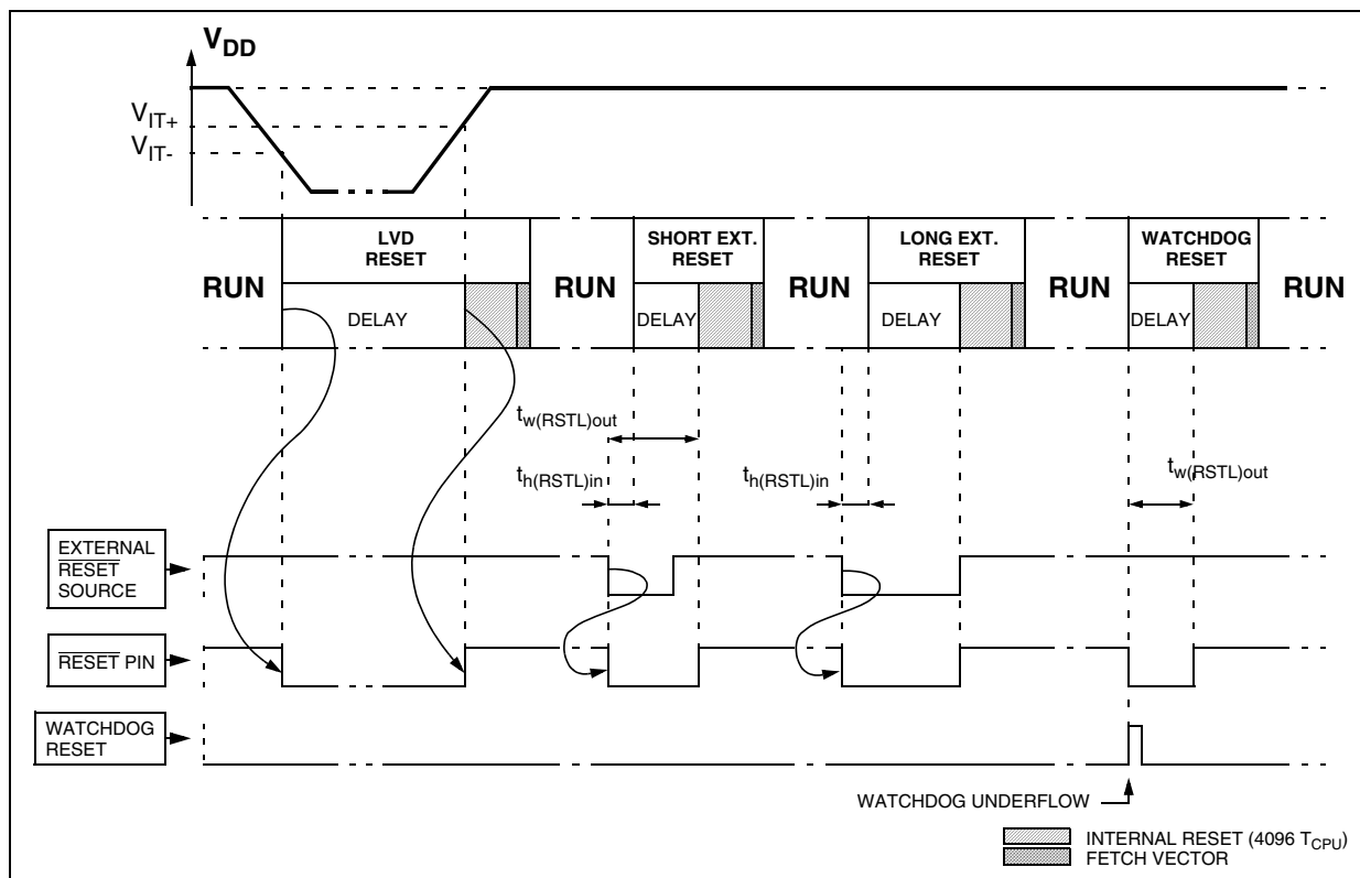
Figure 12. RESET Sequences
