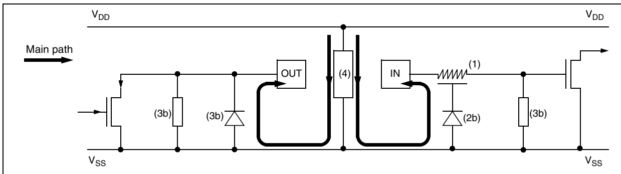
Figure 77. Multisupply Configuration
