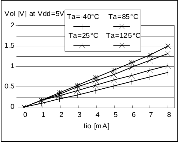
Figure 88. Typical V_{OL} at V_{DD}=5V ( \overline{\text{RESET}} )
