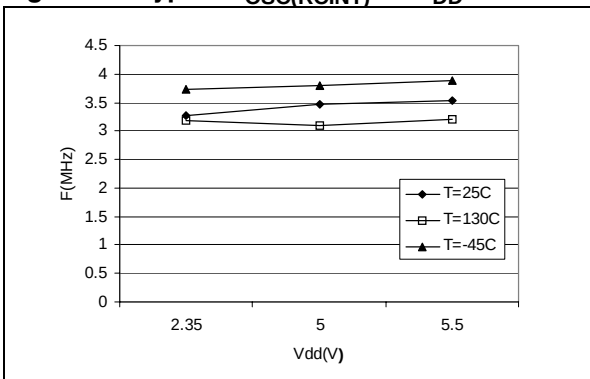
Figure 73. Typical f_{\text{OSC(RCINT)}} vs V_{\text{DD}}
