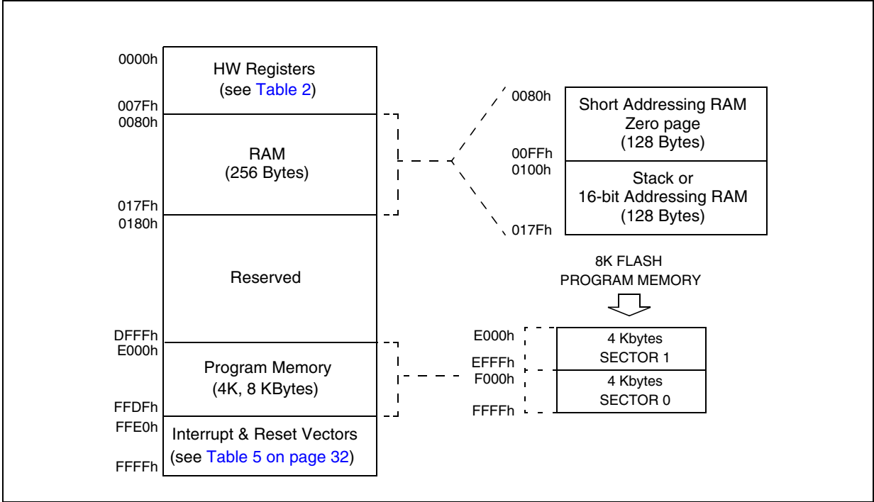
Figure 5. Memory Map
