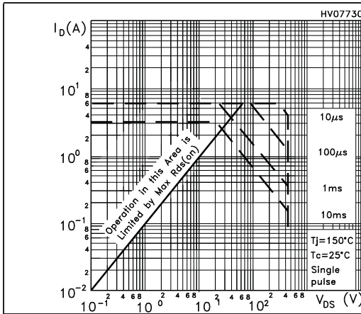
Figure 3. Safe operating area for TO-92
