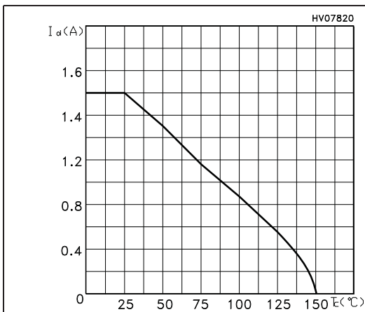
Figure 15. Max Id current vs Temperature
