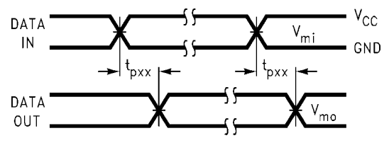
FIGURE 2. Waveform for Inverting and Non-inverting Functions
