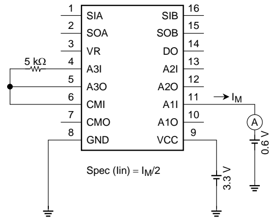
(7) OP-AMP1 Input current: Iin
