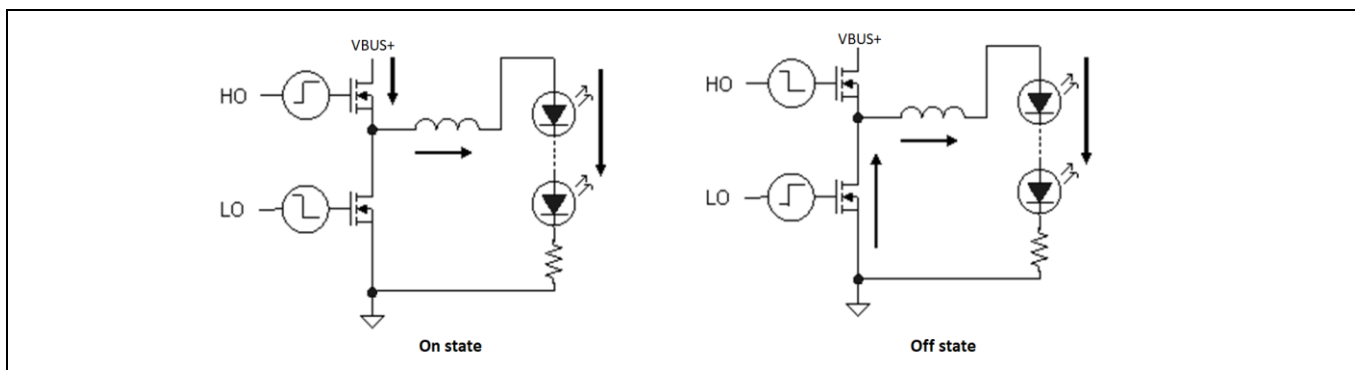
Figure 4 Synchronous buck operation
