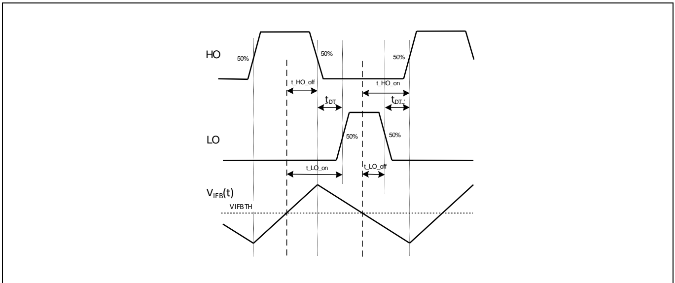
Figure 5 Hysteretic operation
