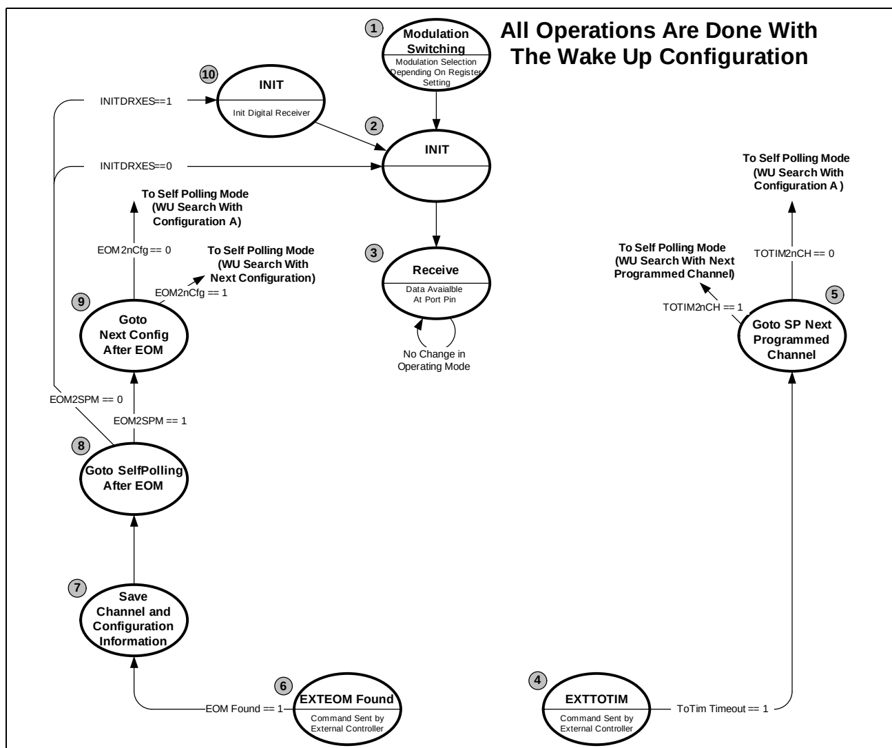
Figure 43 Run Mode Self Polling
