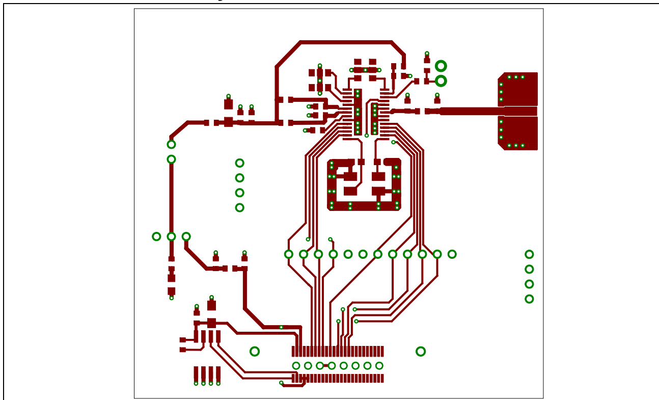
Figure 55 Test Board Layout, Top View
