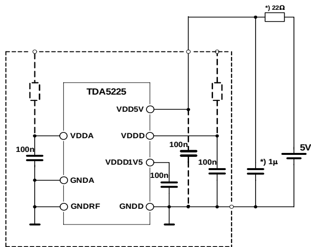
Supply-Application in 5V environment
