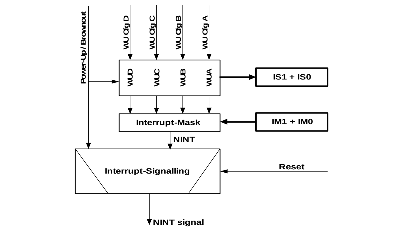
Figure 25 Interrupt Generation Unit
