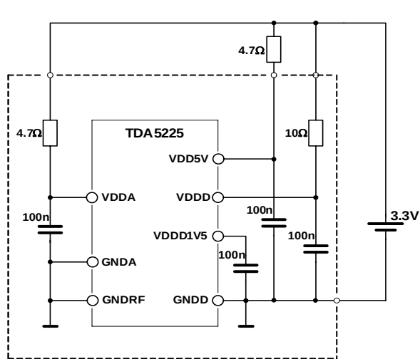
Supply-Application in 3.3V environment
