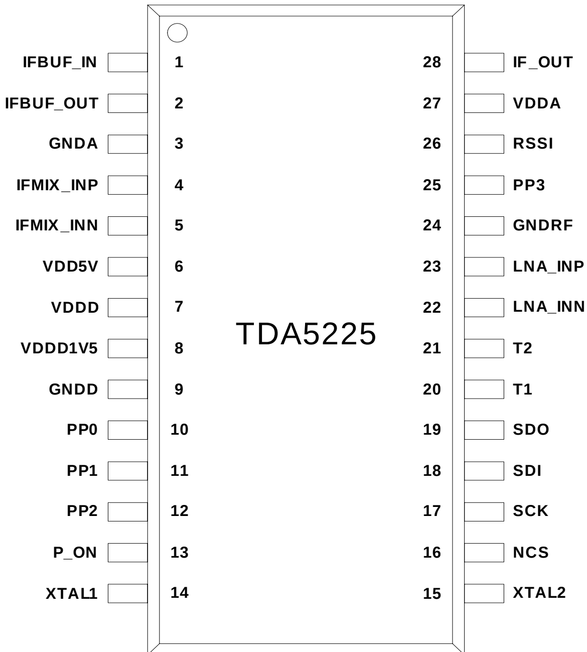
Figure 1 Pin-out
