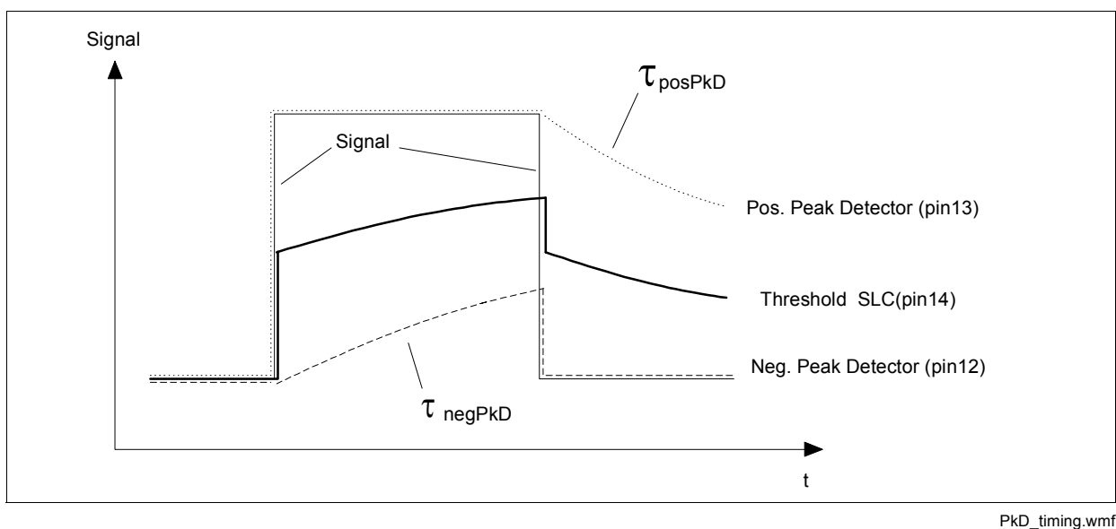
Figure 3-27 Peak Detector timing
