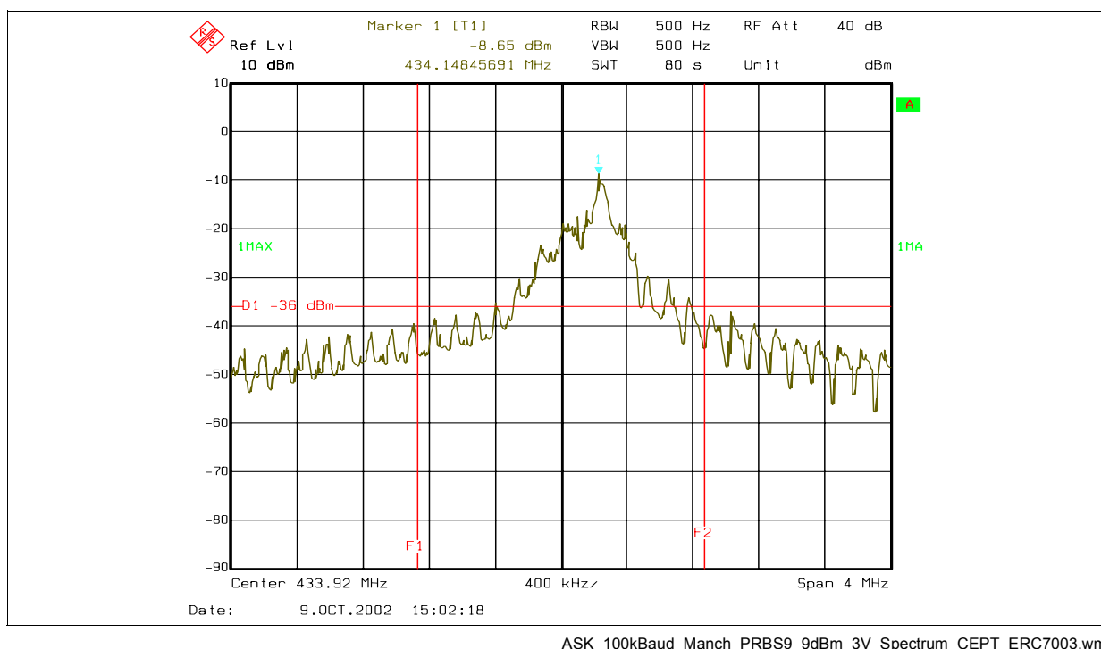
Figure 3-12 ASK Transmit Spectrum 100kBaud, Manch, PRBS9, 9dBm, 3V
