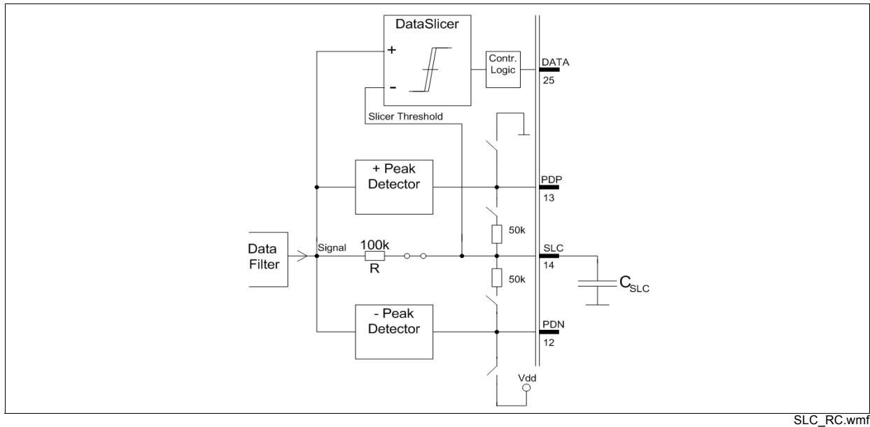
Figure 3-25 Slicer Level using RC Integrator
