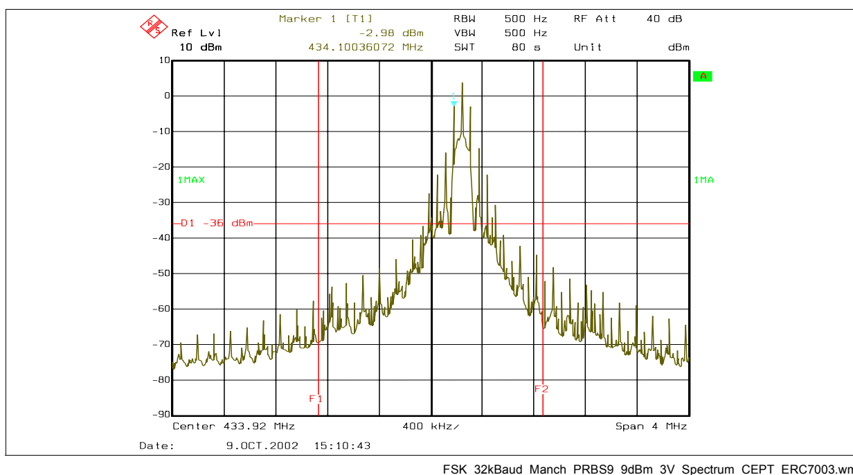
Figure 3-13 FSK Transmit Spectrum 32kBaud, Manch, PRBS9, 9dBm, 3V
