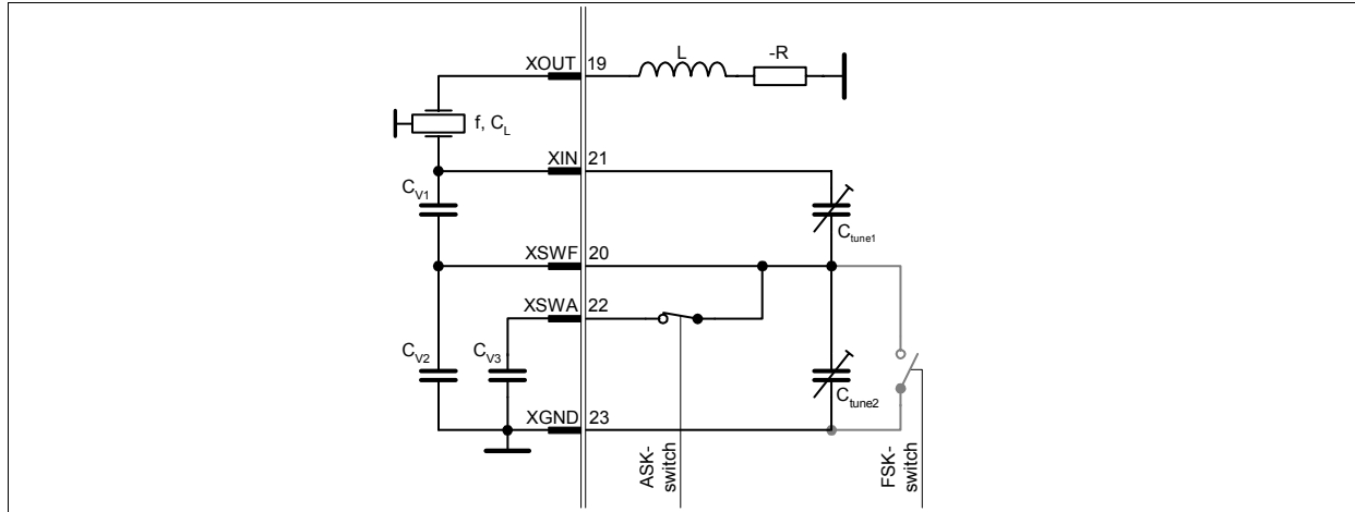
Figure 3-18 FSK receive
