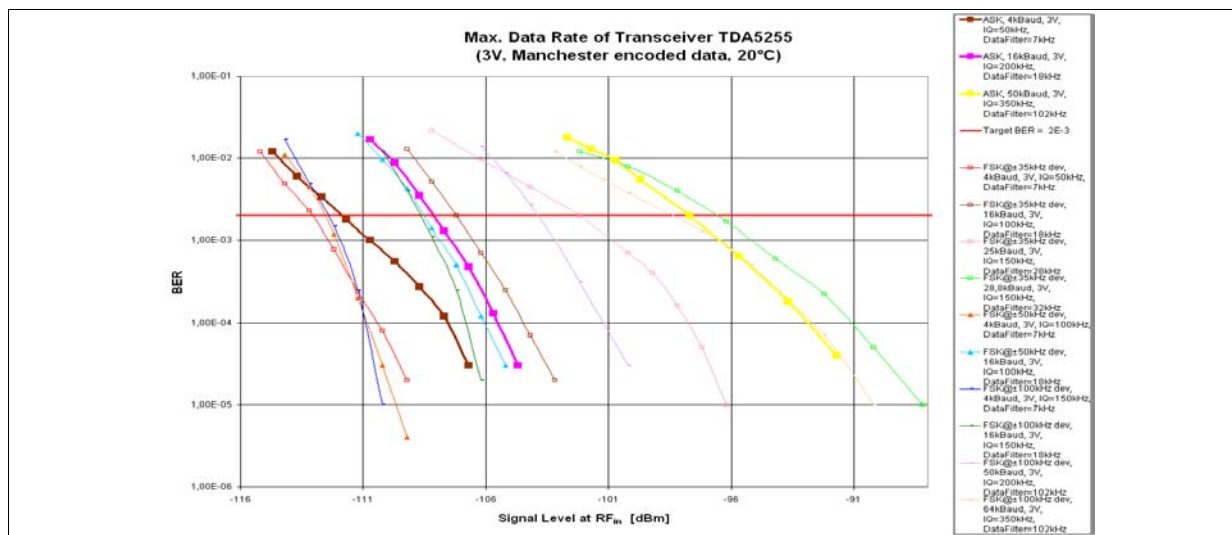
BER Datarate.wmf
