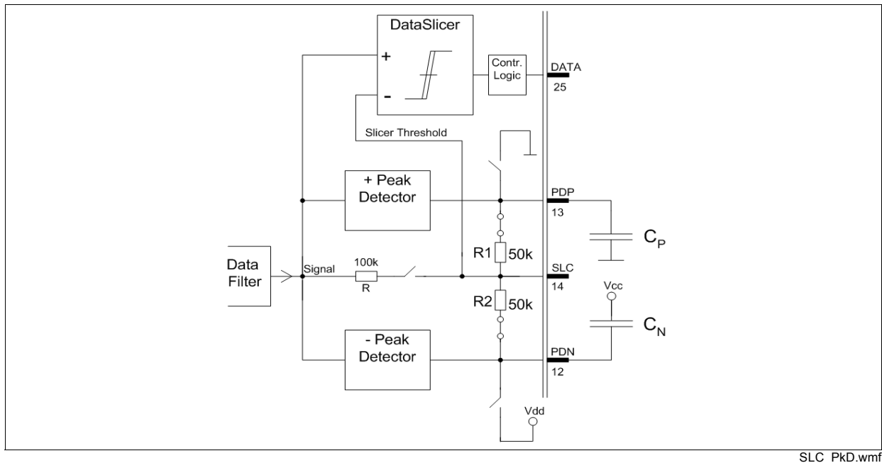
Figure 3-26 Slicer Level using Peak Detector
