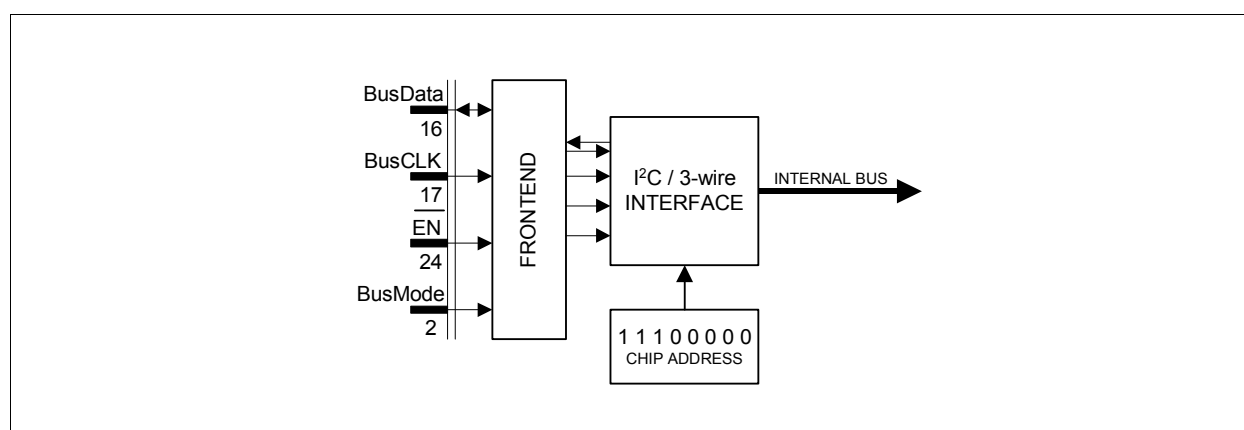
Figure 2-7 Bus Interface
