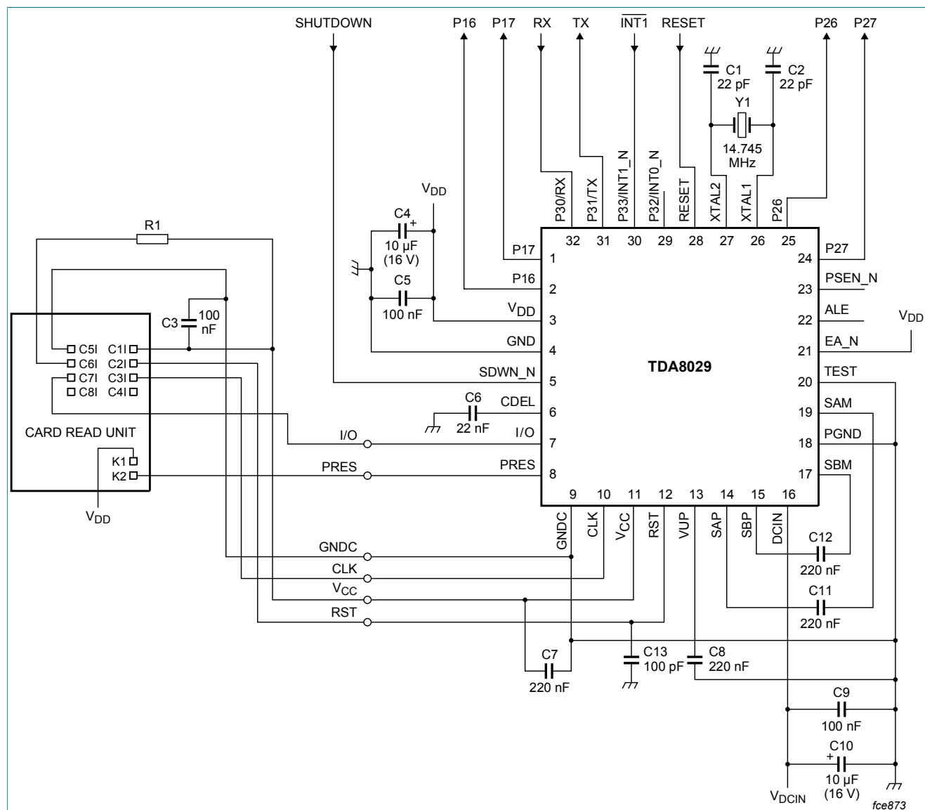
Figure 14. Application diagram
