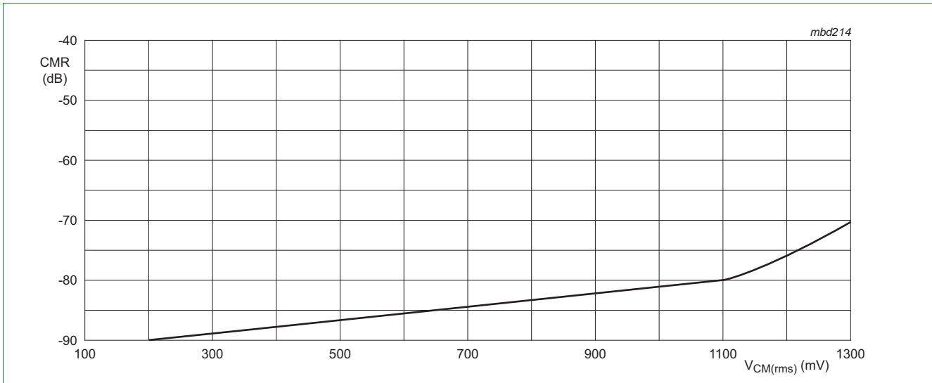
Fig 7. Common-mode rejection ratio as a function of common-mode input voltage; f = 1 \text{ kHz} , R_s = 0 \Omega
