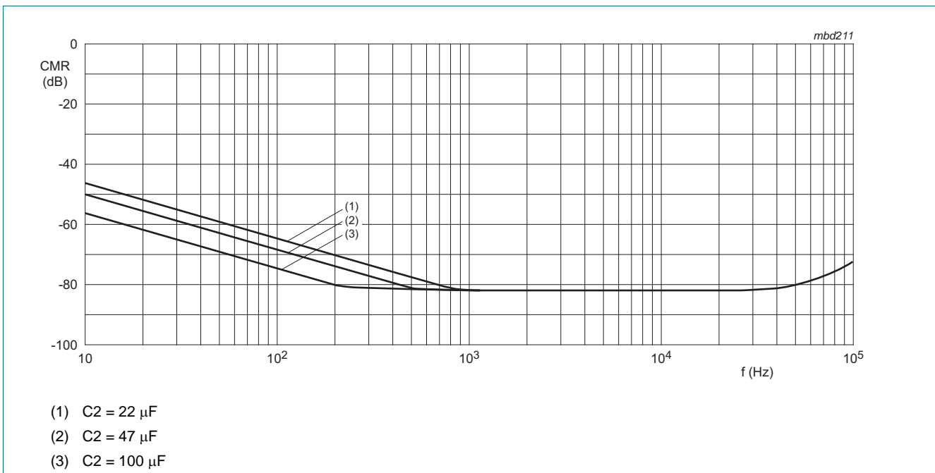
Fig 8. Common-mode rejection ratio as a function of frequency; V_{CM} = 1 \text{ V (RMS)}
