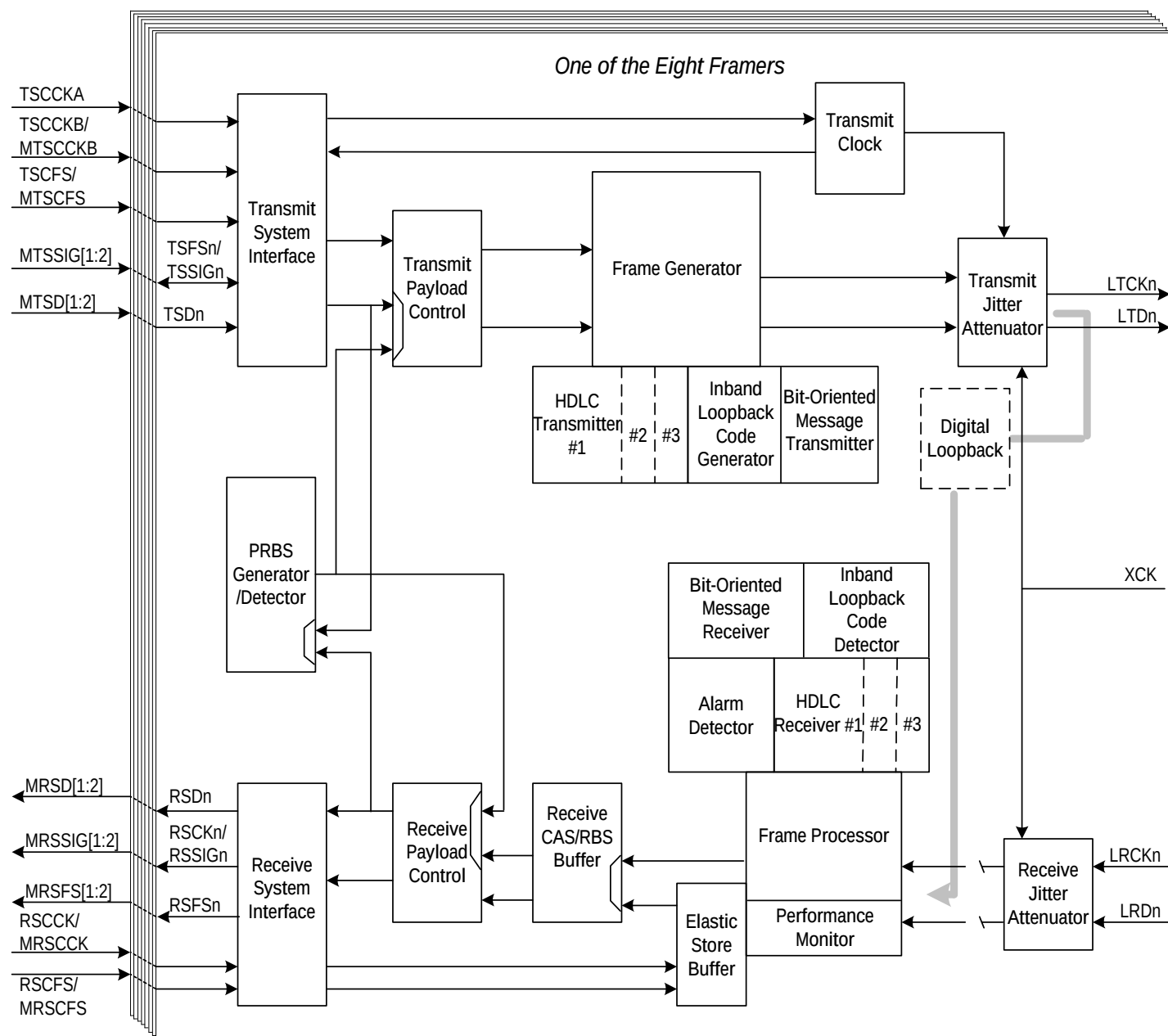
Figure 71. Digital Loopback
