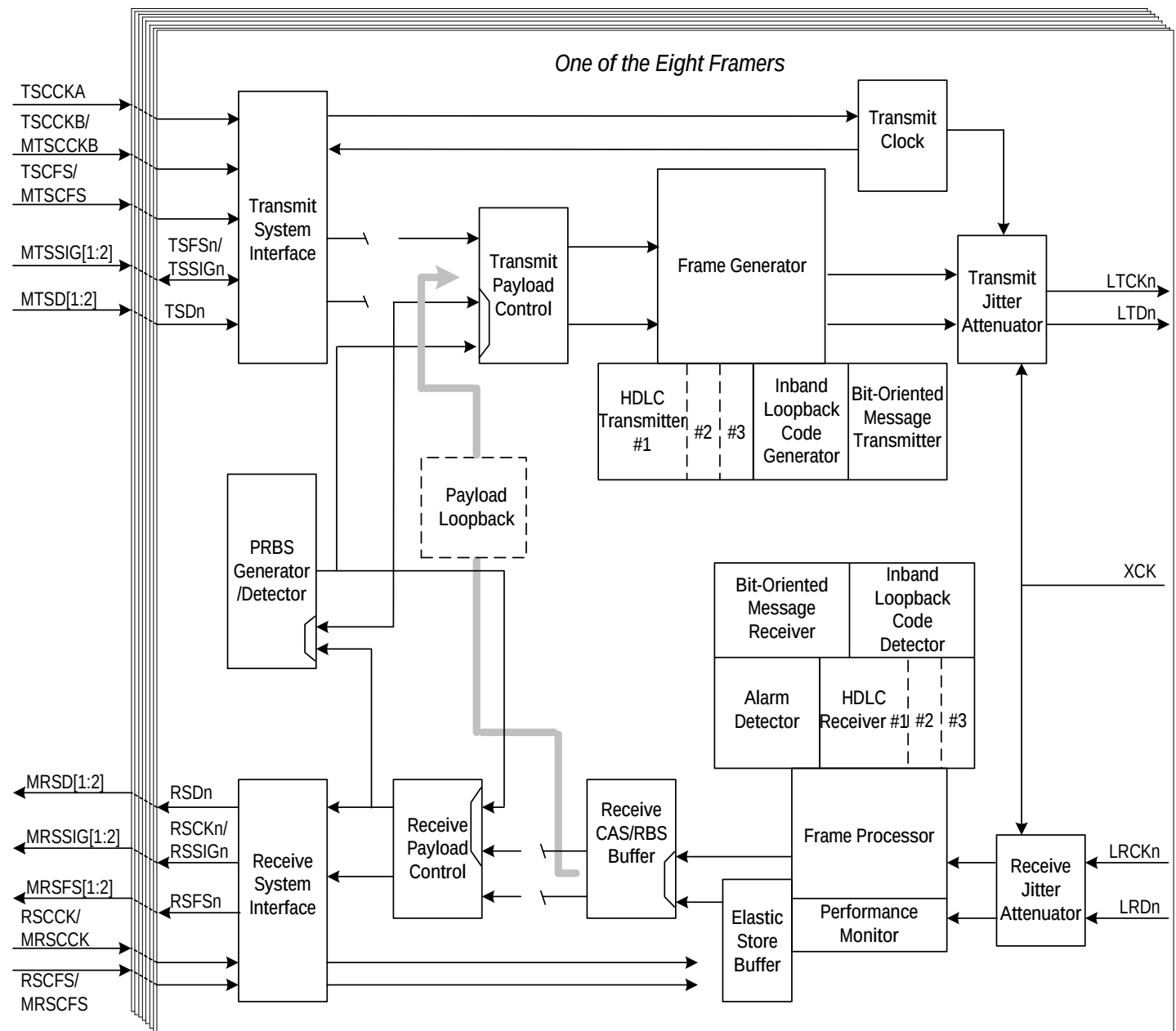
Figure 72. Payload Loopback
