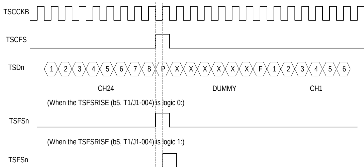
Figure 55. T1/J1 Transmit Clock Slave TSFS Enable Mode - Functional Timing Example 2
