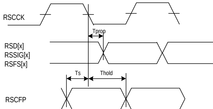
Figure 91. Receive Interface Timing (Receive System Common Clock)
