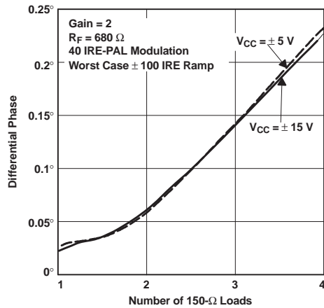
Figure 39. Differential Phase vs Number of 150- \Omega Loads
