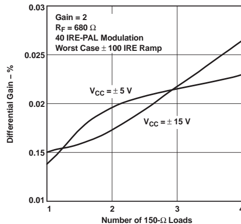
Figure 41. Differential Gain vs Number of 150- \Omega Loads
