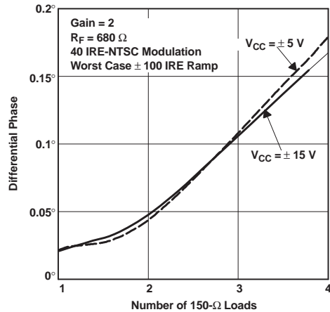
Figure 38. Differential Phase vs Number of 150- \Omega Loads
