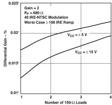
Figure 40. Differential Gain vs Number of 150- \Omega Loads
