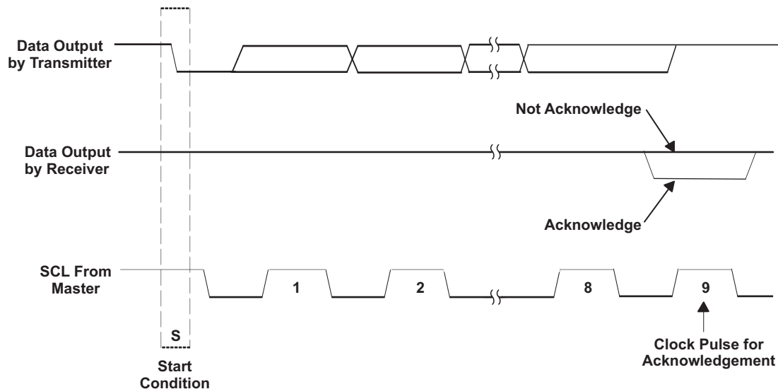
Figure 7. I²C Acknowledge
