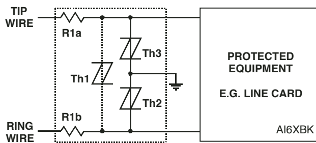
Figure 15. Protection Module
