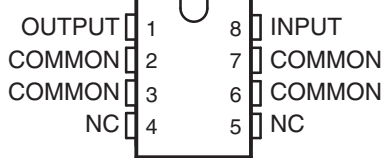
TL750L...D PACKAGE (TOP VIEW)
