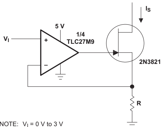
Figure 45. Precision Low-Current Sink
